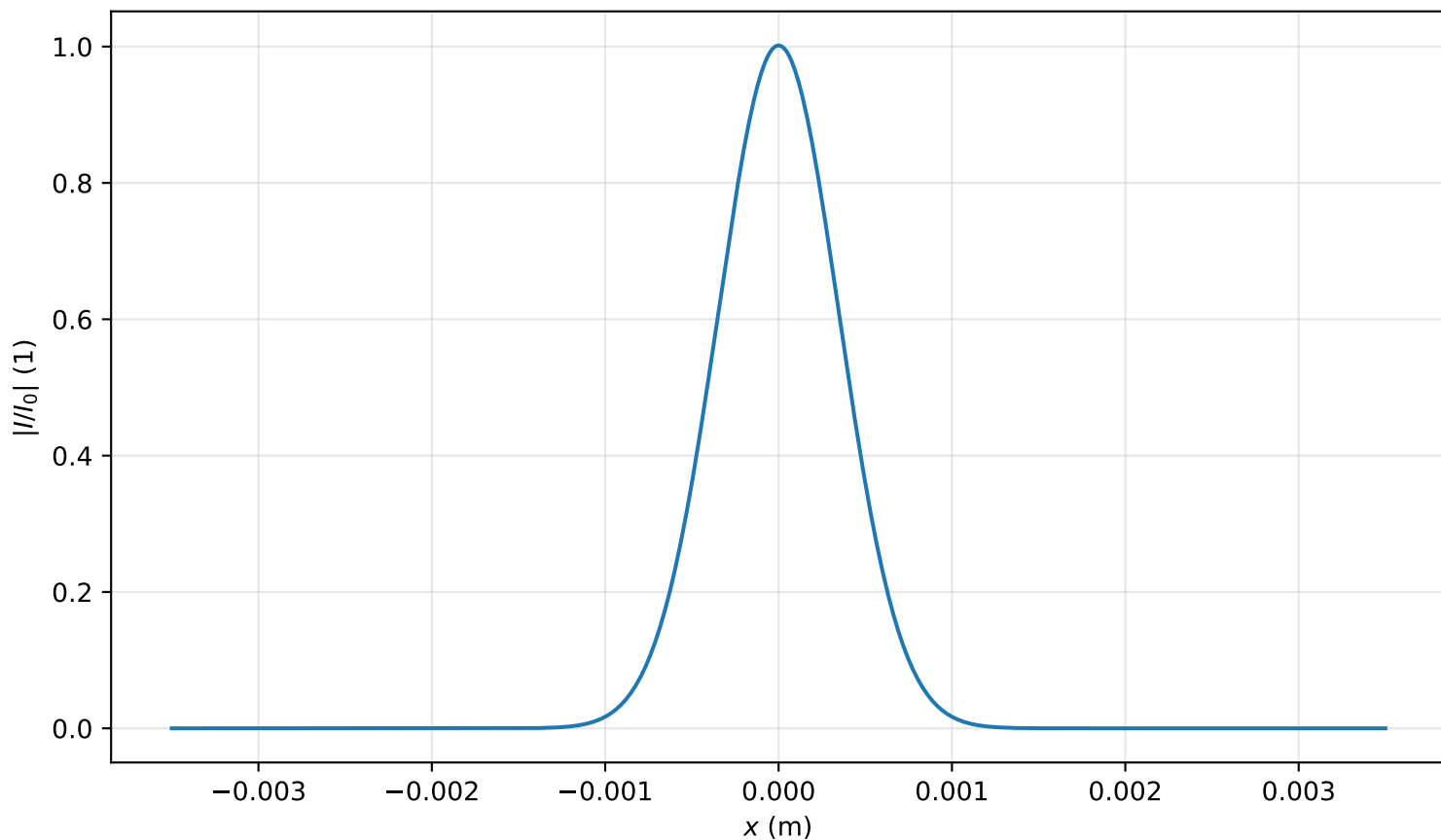
Intensity profile I(x, y = 0, z = 0.080m)/I_0 , P_{in}=0.5P_{cr} , artificial time
